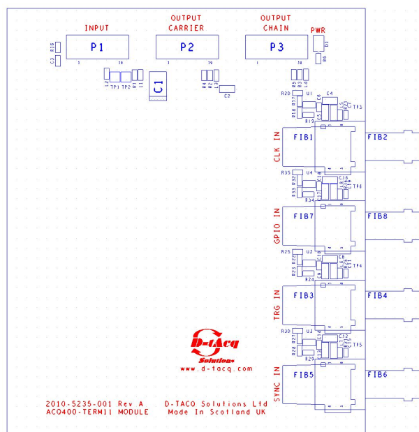
Fig.2 TERM11 PCB layout.
